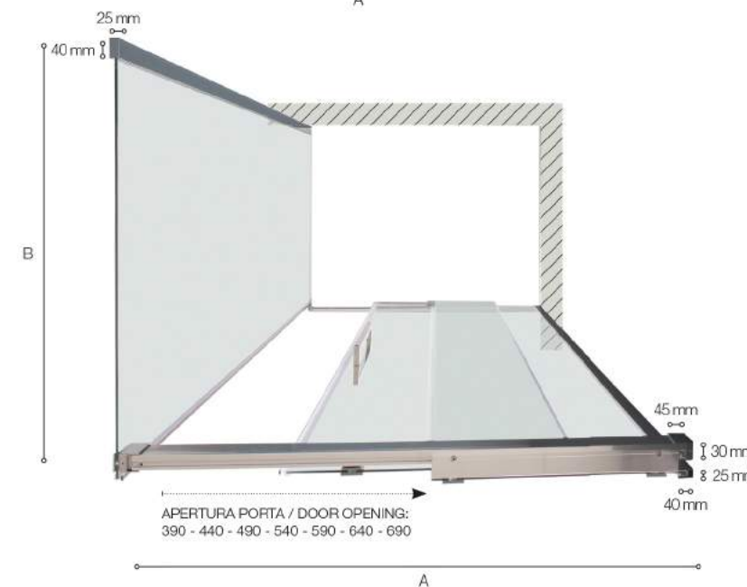
PORTA ABBINATA A LATO FISSO DOOR MATCHED WITH FIXED PANEL
