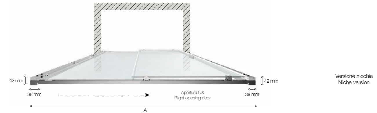
DIMENSIONI PORTA (A) (NICCHIA) DOOR SIZES (A) (NICHE)
