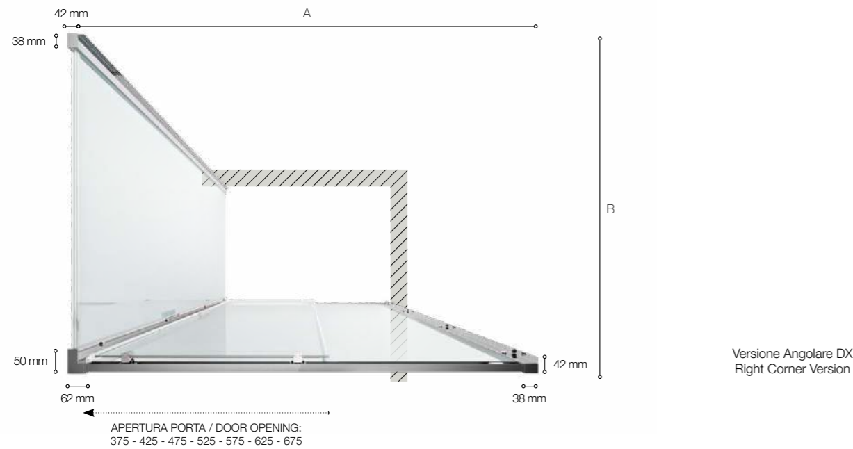
PORTA ABBINATA A LATO FISSO DOOR MATCHED WITH FIXED PANEL
