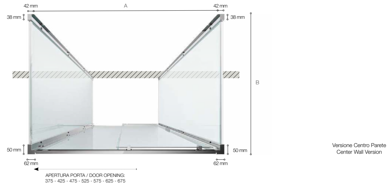
PORTA ABBINATA A 2 LATI FISSI DOOR MATCHED WITH 2 FIXED PANELS
