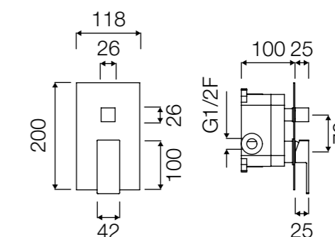
HKINC142C Incasso doccia quadro Recessed square shower control
