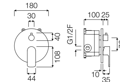
HKINC143C Incasso doccia tondo Recessed round shower control
