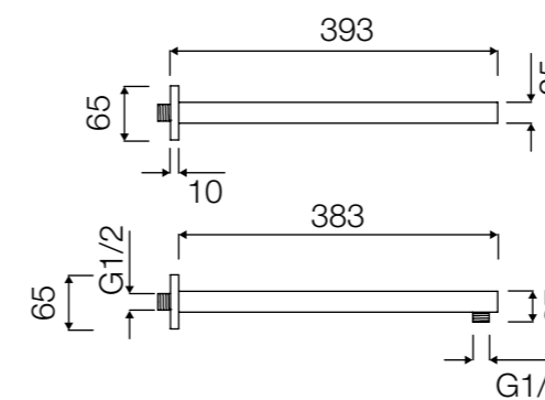
HKAST110C Asta a muro quadra Square wall-mounted shower arm
