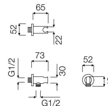
HKSUP121C Supporto doccetta tonda Round handheld showerhead holder
